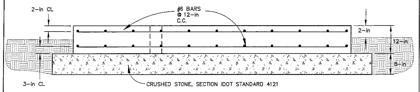
DETAIL 1-FOUNDATION
